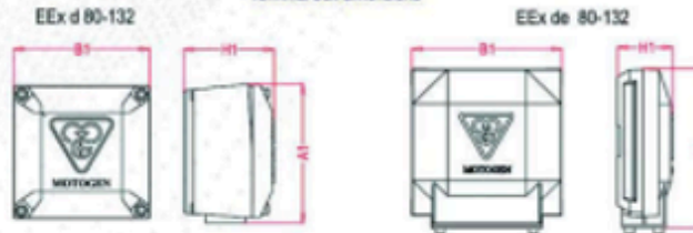
Terminal box dimensions
