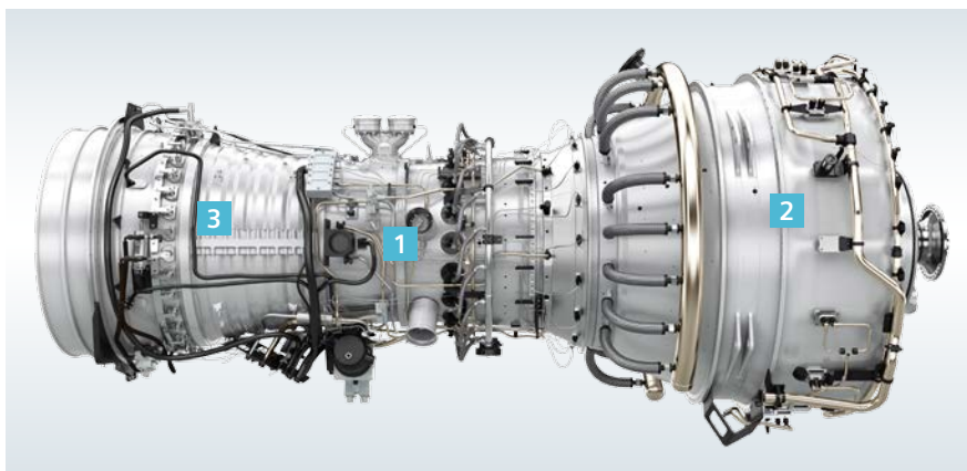
Lightweight architecture of the SGT-A35 (GT30) gas turbine
